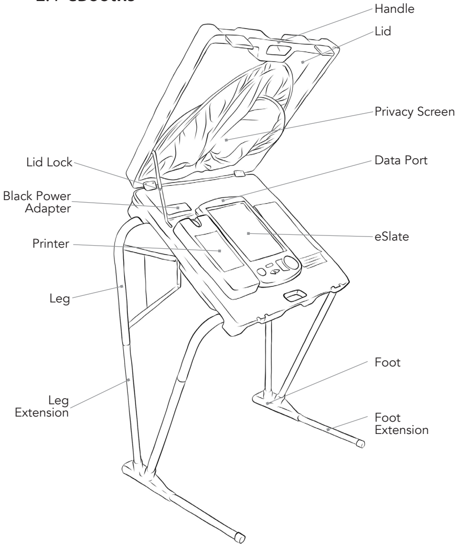
Full view of eBooth.
